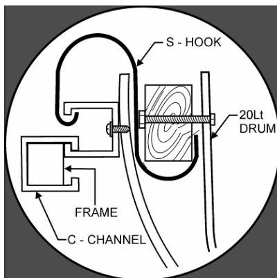
Detail of side elevation as marked in photo above.
